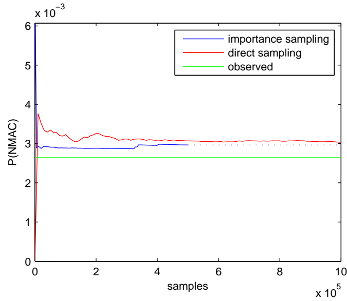
Figure D-2. Convergence curves for importance and direct sampling. Also shown is observed P(\text{NMAC}) .
