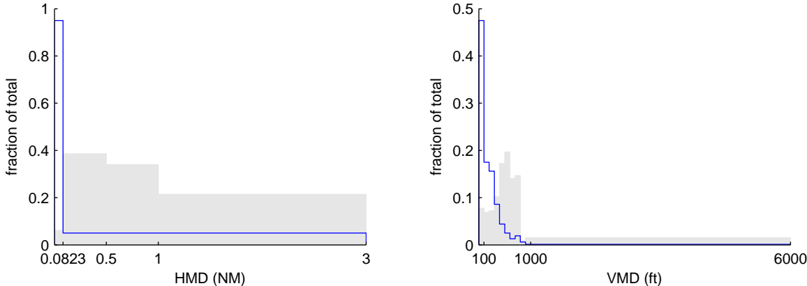
Figure D-1. Histograms of hmd (left) and vmd (right). The sampling distribution is outlined in blue, the observed distribution is shaded.
