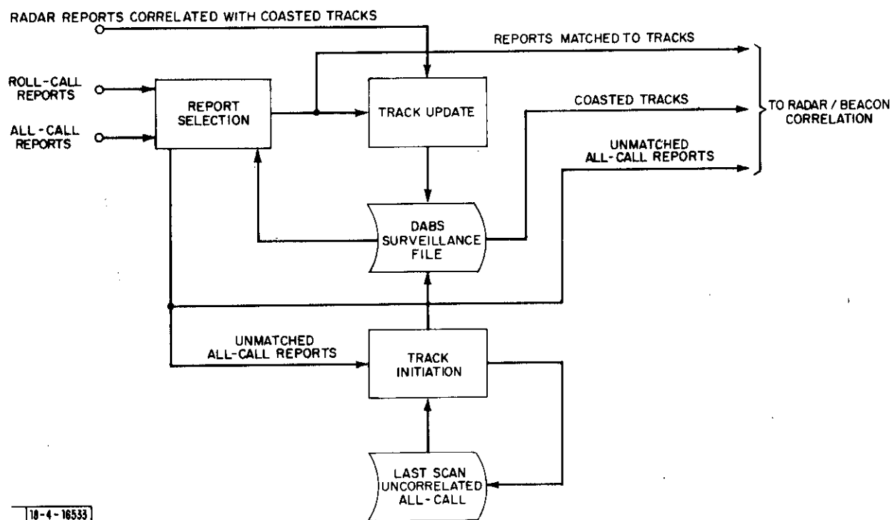
Fig. 3-13. Surveillance Processing
