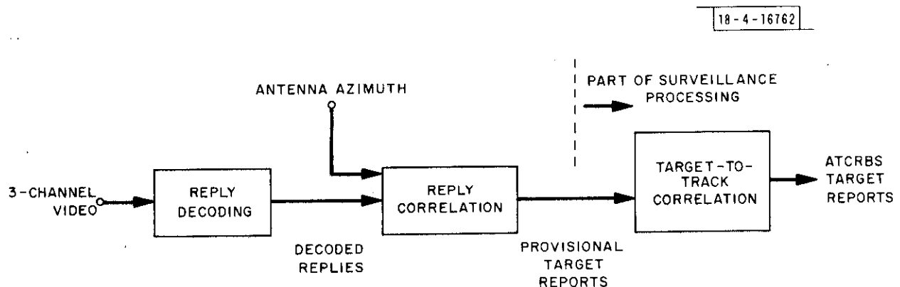
Fig. 3-11. ATCRBS Reply Processing.
