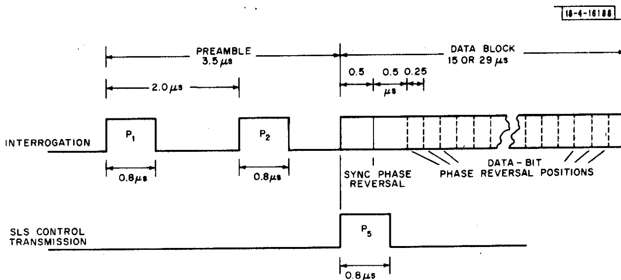
Fig. 2-3. DABS Interrogation.
