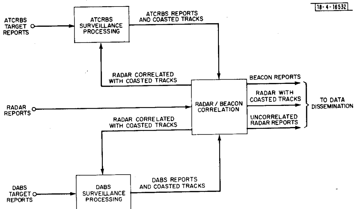
Fig. 3-13. Surveillance Processing
