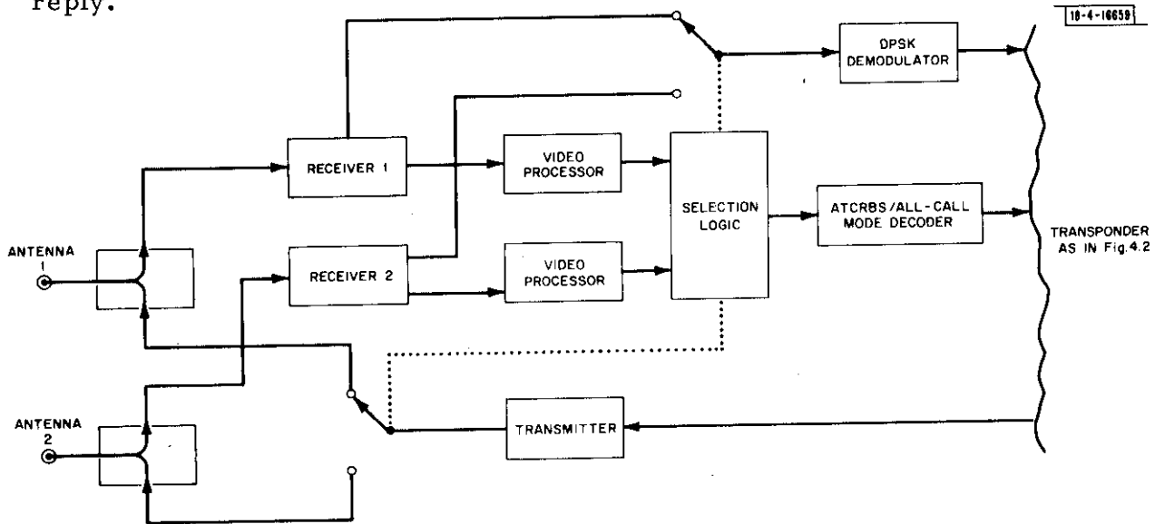
Fig. 4-3. Diversity Transponder
