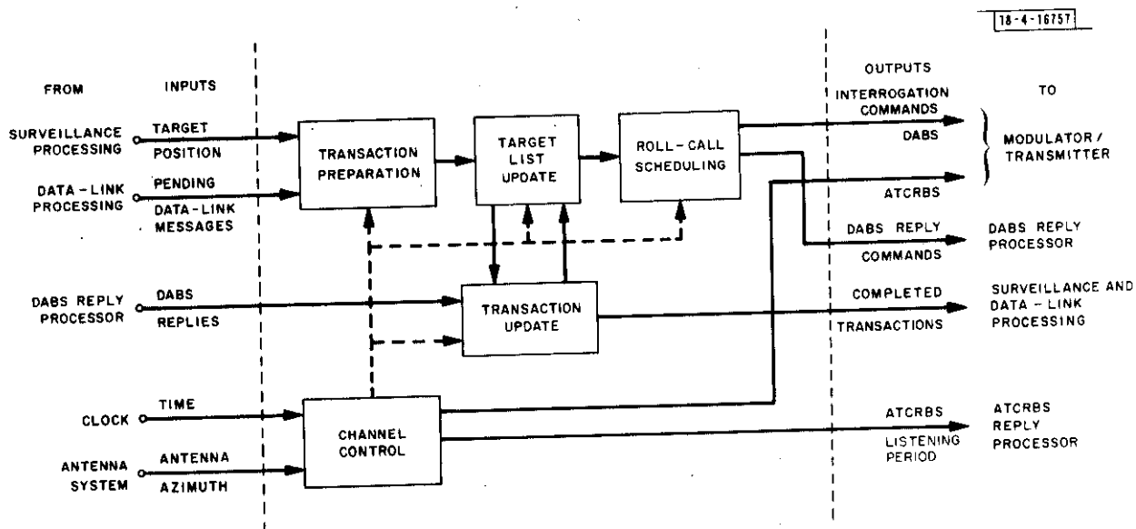
Fig. 3-5. Channel Management.
