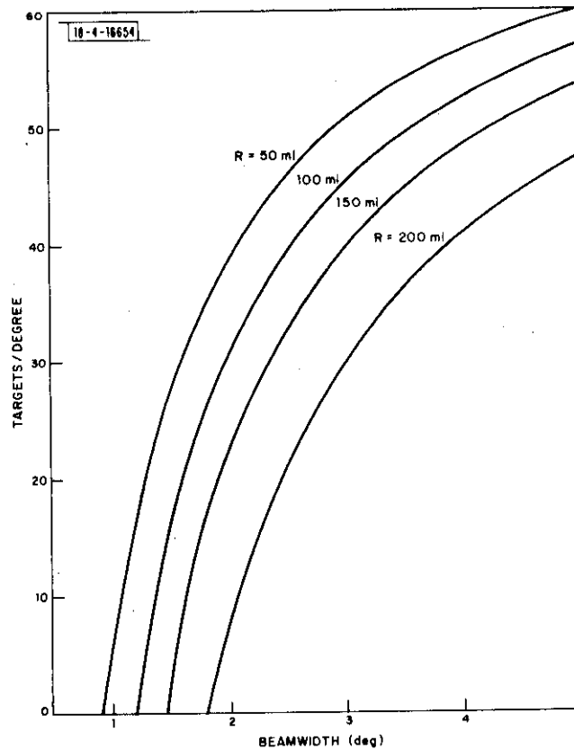
Fig. 5-8. Capacity plots.
