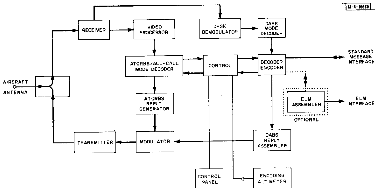
Fig. 4-2. DABS Transponder
