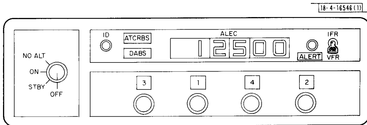
Fig. 4-1. Transponder Panel
