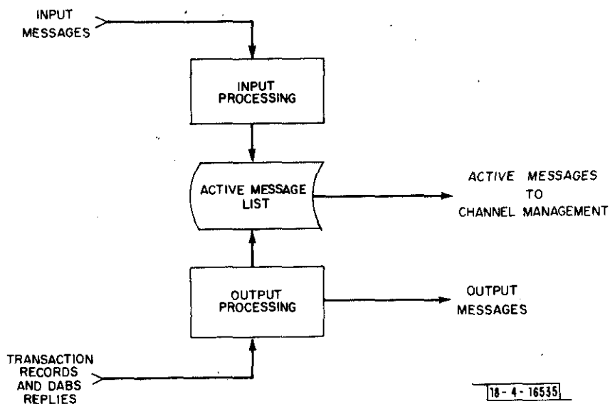
Fig. 3-16. Data-Link Processing
