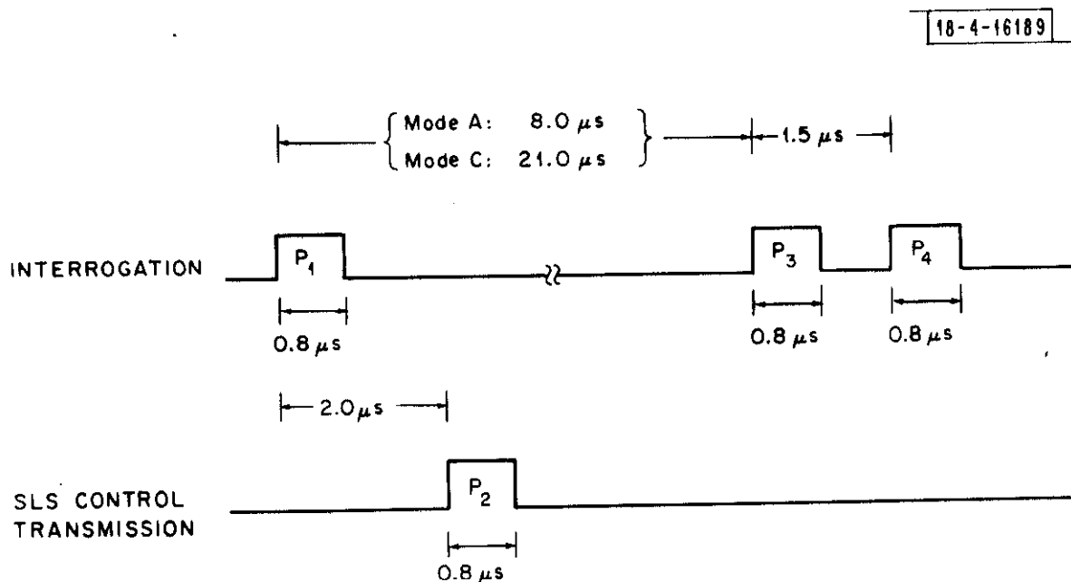
Fig. 2-1. ATCRBS/DABS All-Call Interrogation.
