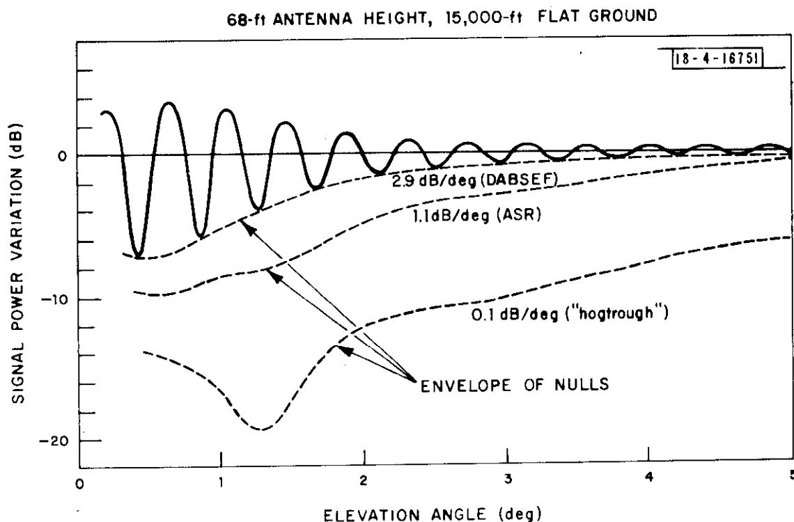
Fig. 5-1 Vertical Lobing
