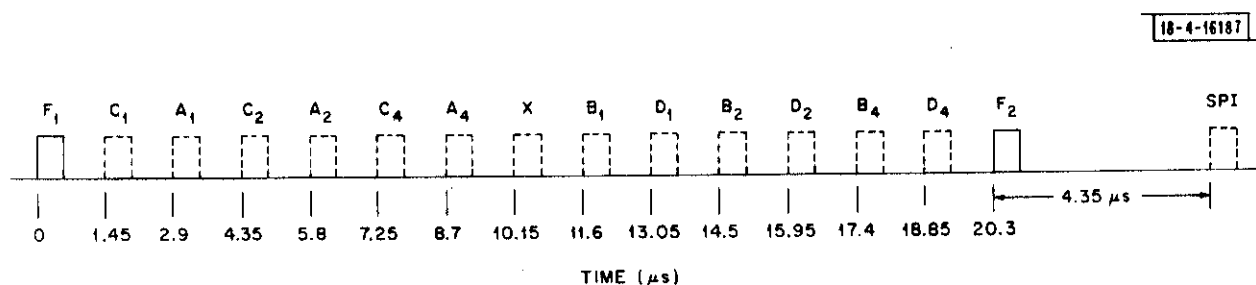
Fig. 2-2. ATCRBS Reply.
