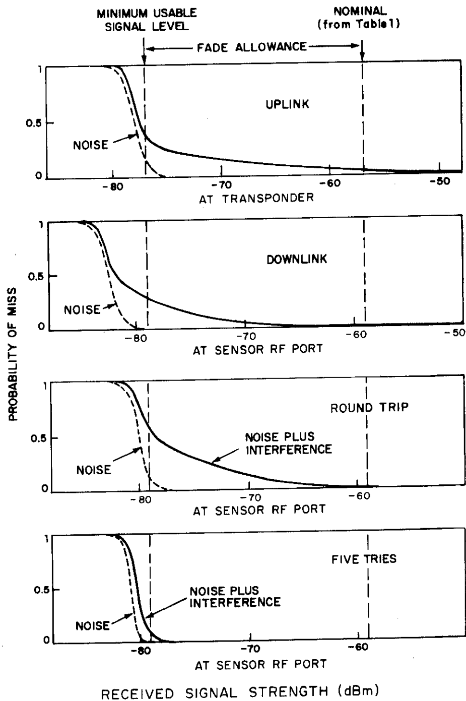
Fig. 5-3. Miss Probability.
