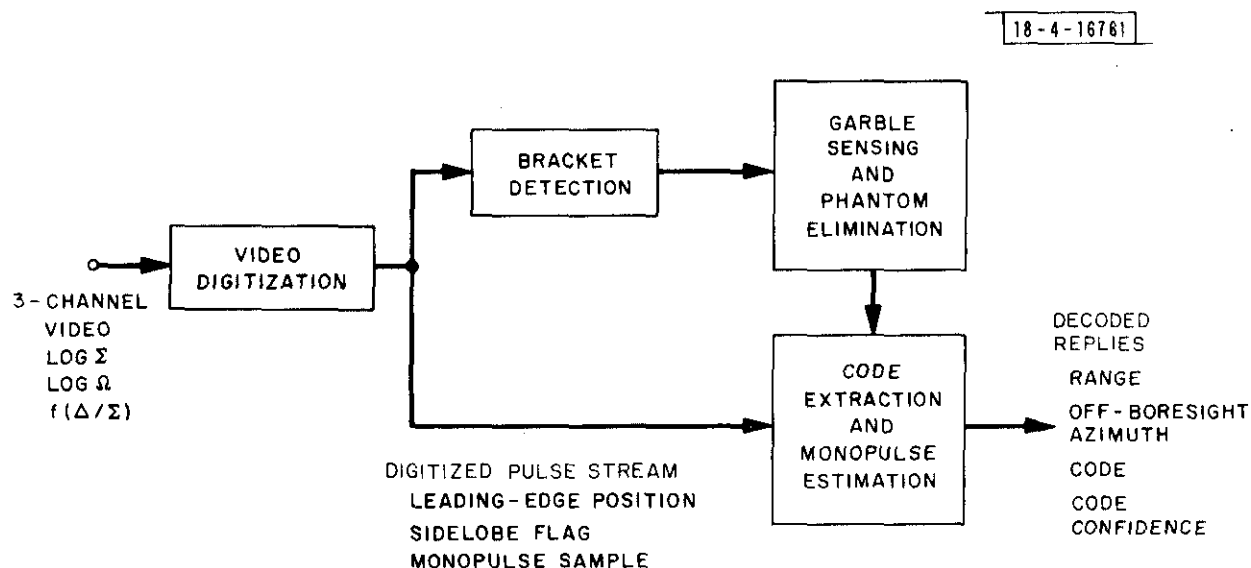
Fig. 3-12. ATCRBS Reply Decoding.
