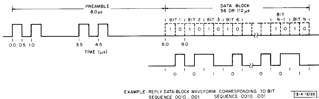
Fig. 2-4. DABS Reply
