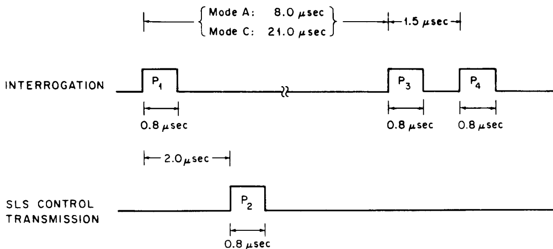
Fig. 2.3-1. ATCRBS/DABS All-Call interrogations.
