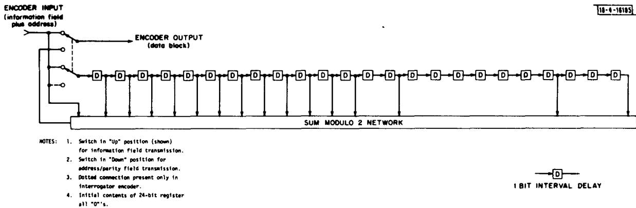
Fig. 5.4-1. Functional diagram of DABS interrogator and transponder encoders.
