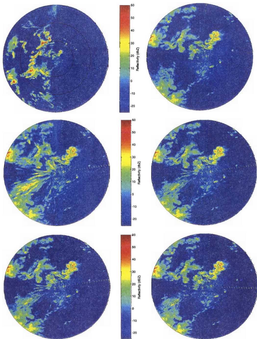
Figure 10. Reflectivity estimates for (a) PRF = 500 Hz, full 300-km range displayed, (b) PRF = 500 Hz, only first 100 km shown, (c) PRF = 1500 Hz, random phase coding, no phase code processing, (d) PRF = 1500 Hz, random phase coding, phase code processing with low-PRF data, (e) PRF = 1500 Hz, random phase coding, phase code processing without low-PRF data, and (f) PRF = 1500 Hz, SZ(8/64) phase code processing.
