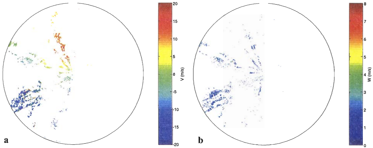
Figure 14. SZ(8/64) phase code processing censored estimates (weak-trip recovery gates only) for (a) velocity and (b) spectral width.
