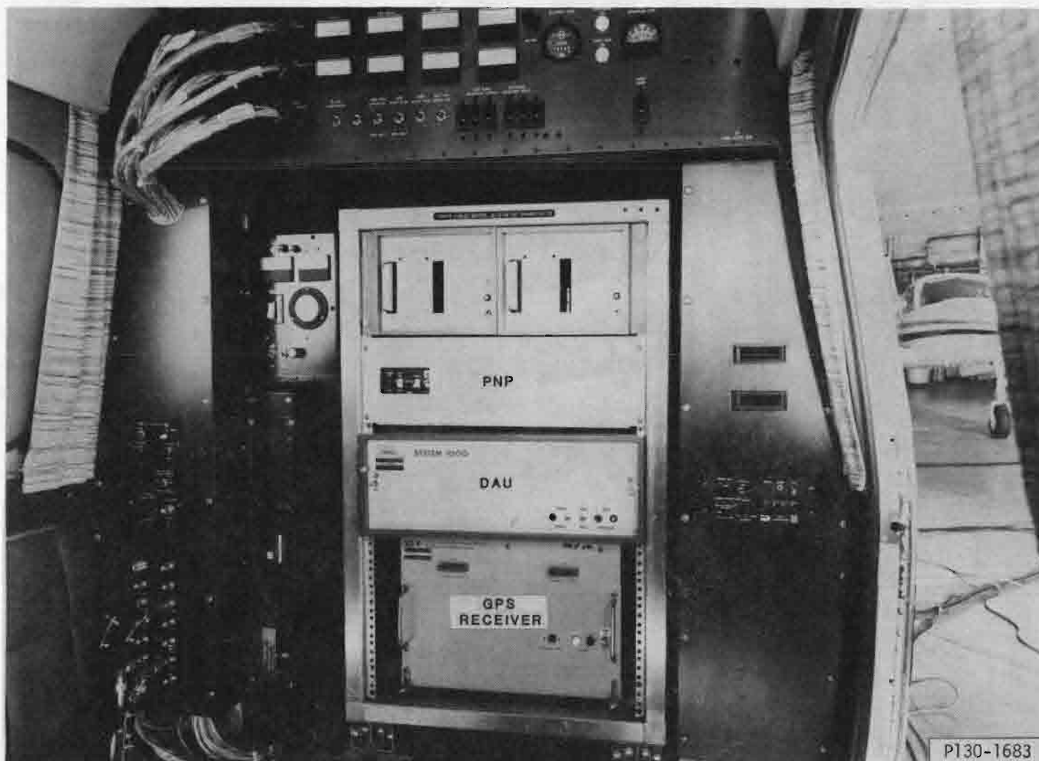
FIG. 4-6. RECEIVER RACK
