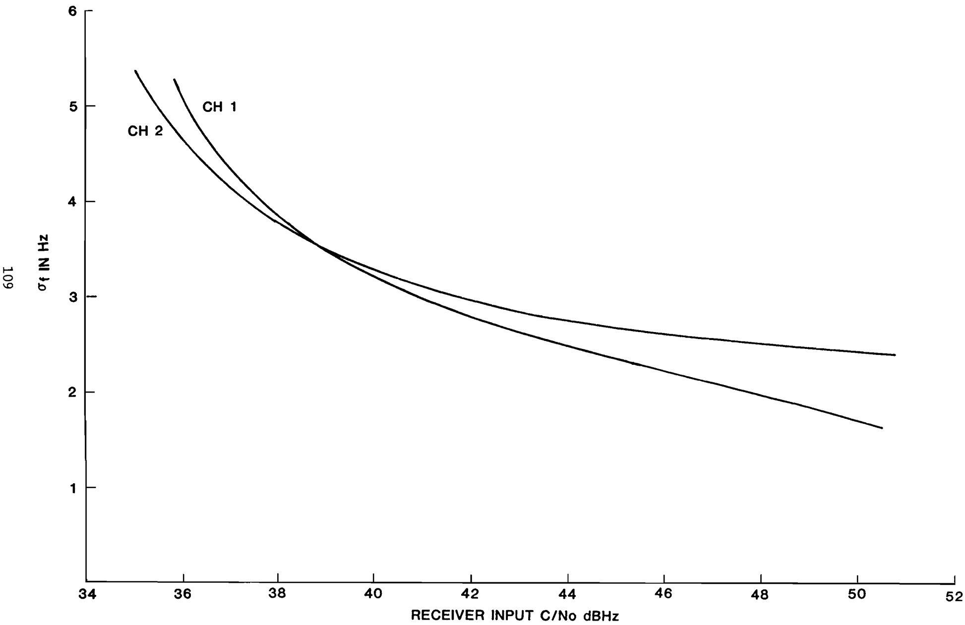
FIG. 4-20. RECEIVER AFC PERFORMANCE IN PHASED TRANSITION
