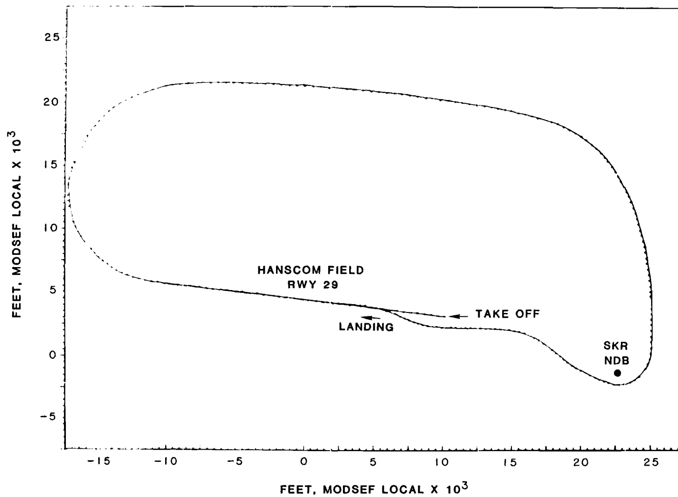
FIG. 4-35. FLIGHT TEST, 21 DEC 82
