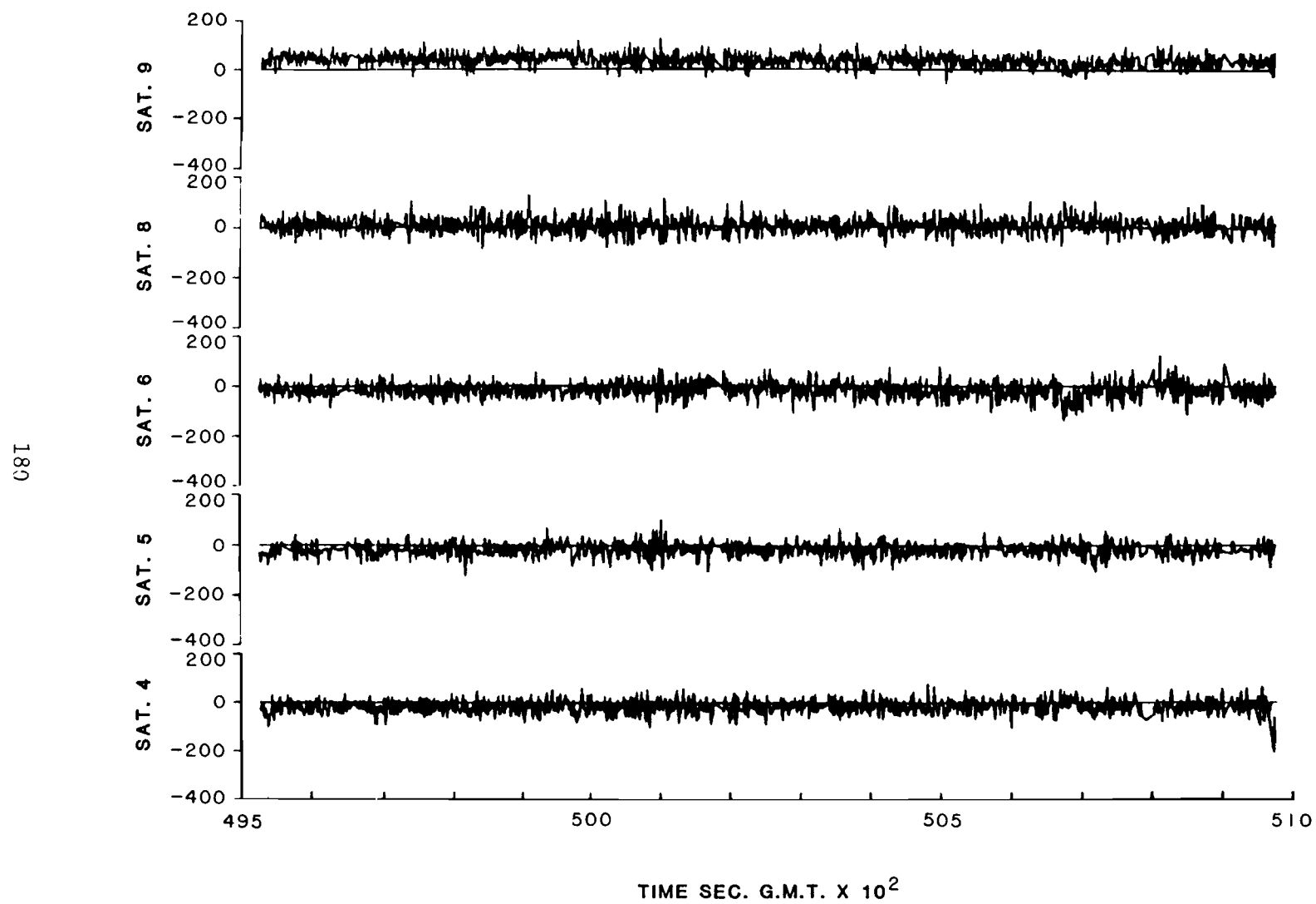
FIG. 4-69. PSEUDO-RANGE RESIDUALS, 25 JAN 83, RUN 2
