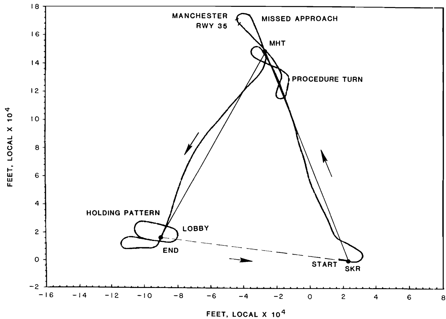
FIG. 4-80. OPERATIONAL TEST, 4 FEB 83, RUN 1a
