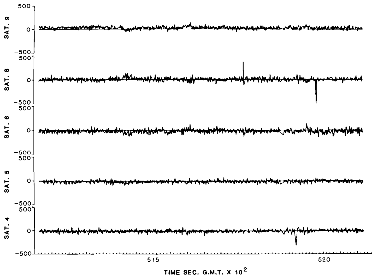
FIG. 4-78. PSEUDORANGE RESIDUALS, 25 JAN 83, RUN 3
