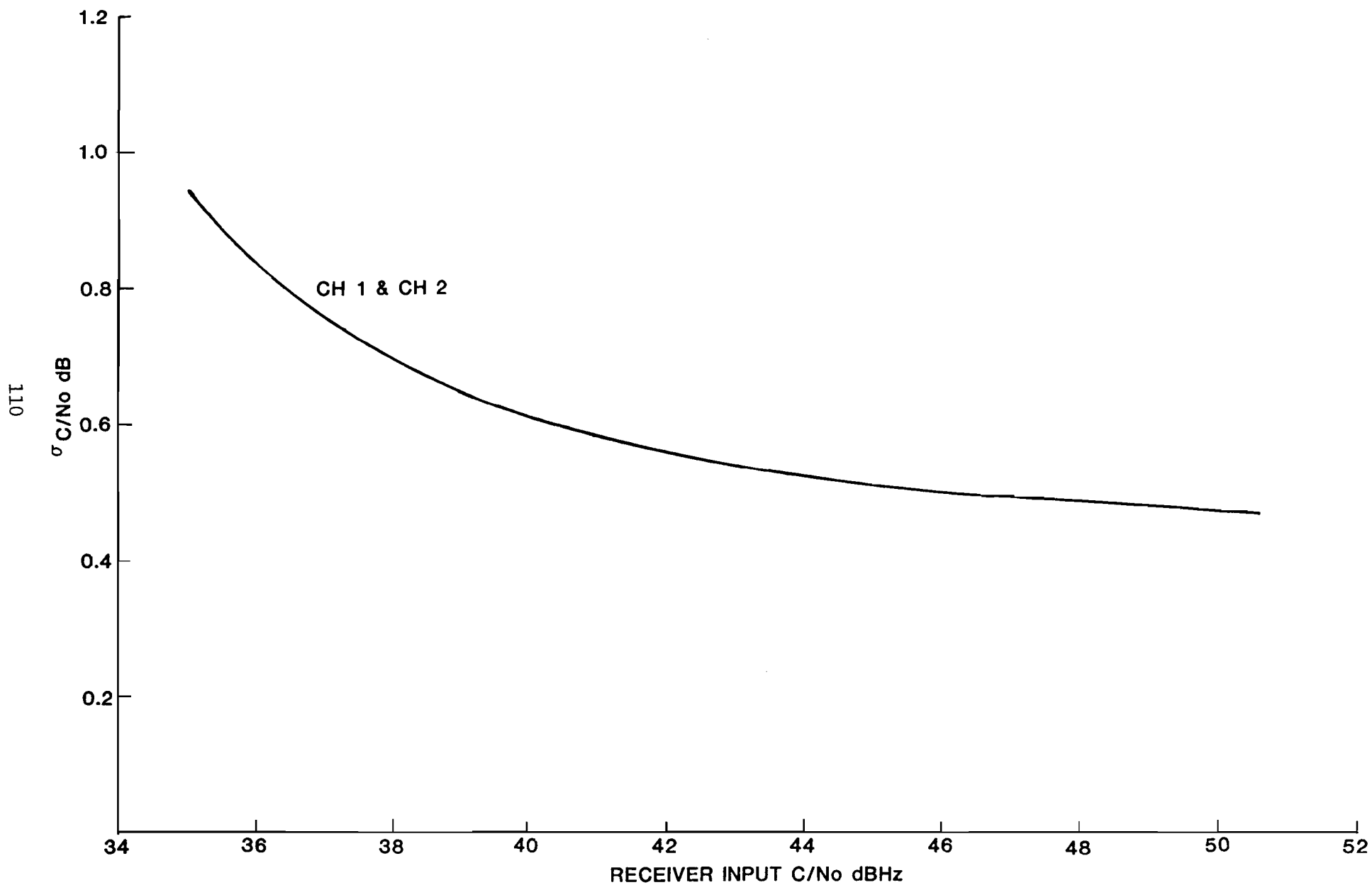
FIG. 4-21. RECEIVER C/No ESTIMATOR PERFORMANCE IN PHASED TRANSITION
