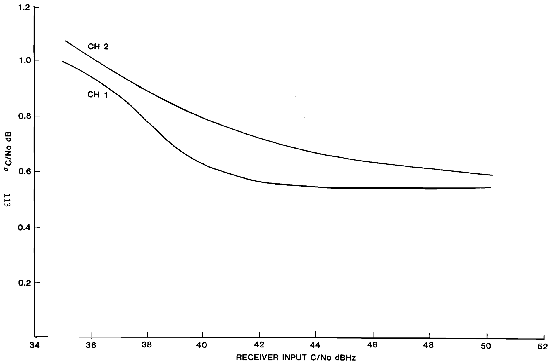
FIG. 4-24. RECEIVER C/N 0 ESTIMATOR PERFORMANCE IN NAVIGATION STATE
