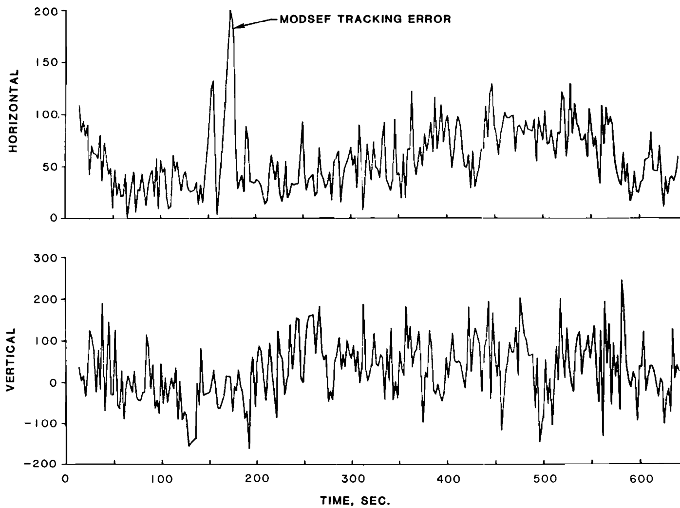
FIG. 4-36a. POSITION FIX ERRORS, 21 DEC 82 FLIGHT TEST
