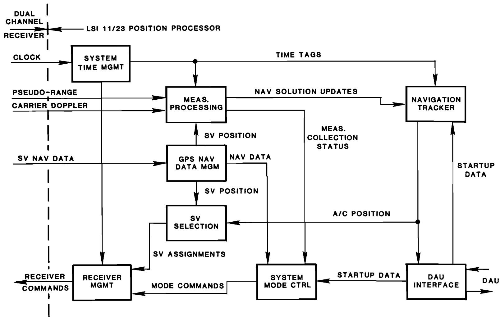
FIG. 3-24. POSITION SOFTWARE SYSTEM BLOCK DIAGRAM
