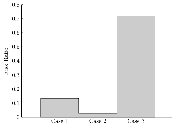
Figure 8. Risk ratio for full encounter set. Case 1: Multi-threat encounters; Case 2: Independently resolved encounters; Case 3: Multi-threat logic off.
