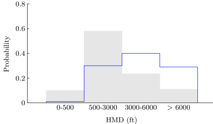
Figure 6. HMD distributions. Solid gray distributions are for Aircraft 1 - Aircraft 2 encounters and the blue line is for Aircraft 1 - Aircraft 3 encounters.
