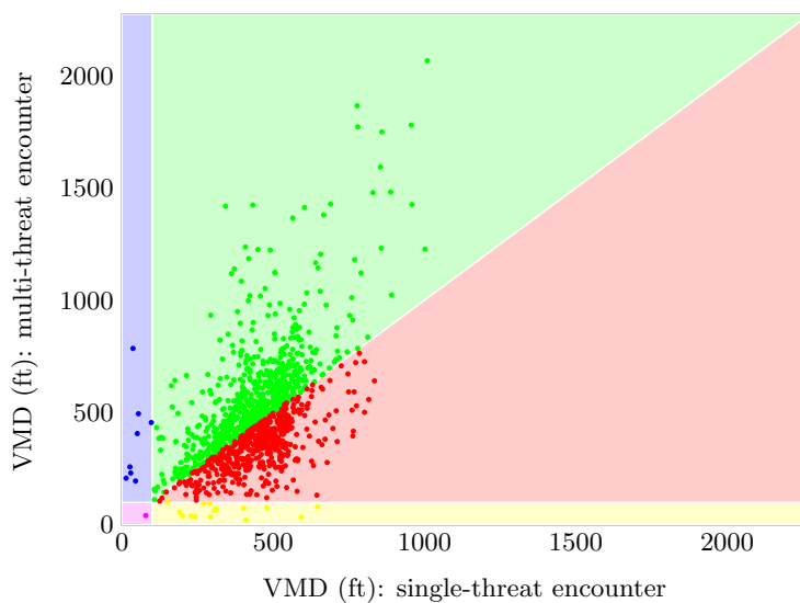
Figure 7. Vertical miss distance between Aircraft 1 and Aircraft 2 for single-threat encounters vs. multi-threat encounters. Approximately 4,000 samples are shown where VMD for single-threat encounters is different from that of multi-threat encounters, but the pattern is reflective of complete encounter set. VMD is defined at the point of minimum horizontal separation between Aircraft 1 and Aircraft 2.
