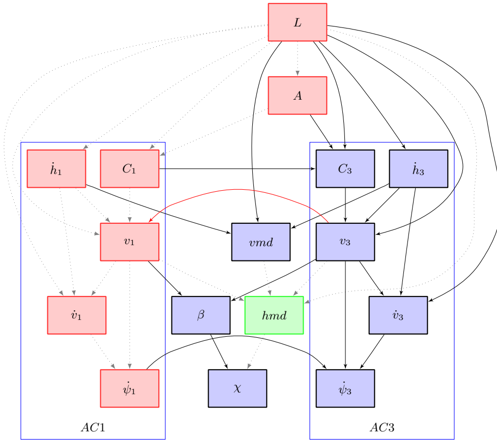
Figure 4. First multi-threat encounter model graphical structure designed to generate Aircraft 3 trajectories that are below Aircraft 1. The red arrows highlight arcs reversed from the original graphical structure. Dotted arrows denote that the original dependency is no longer used to assign variables for the multi-threat encounter. Red nodes indicate that the variable is not sampled, but is rather held fixed. Green nodes indicate that the distribution of the variable is modified to reflect multi-threat encounter characteristics.
