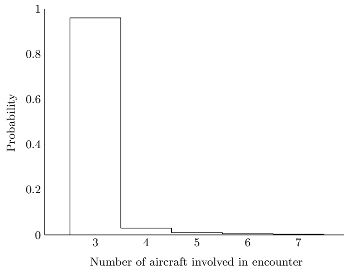
Figure 2. Distribution over the number of aircraft involved in a multi-threat encounter. Over 95% involve three aircraft, but one involved seven aircraft.
