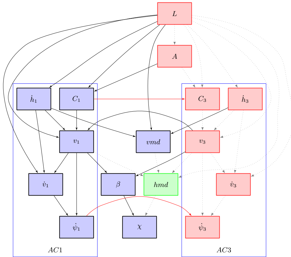
Figure 5. Second multi-threat encounter model graphical structure designed to generate Aircraft 3 trajectories that are above Aircraft 1.
