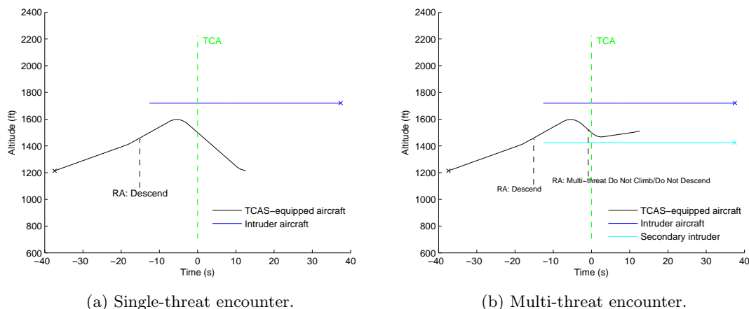
Figure 9. Example simulated single-threat encounter compared to same encounter with additional threat. Aircraft 1 equipped with TCAS, Aircraft 2 and Aircraft 3 equipped with Mode S transponders.
