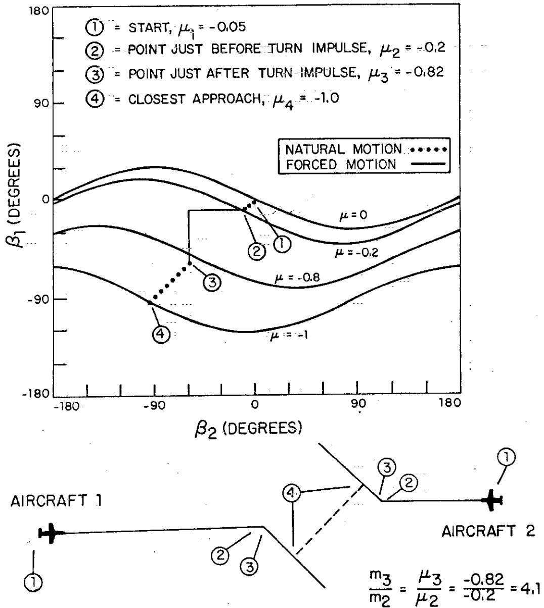
Fig.A-3. An encounter plotted as a combination of natural and forced motion.
