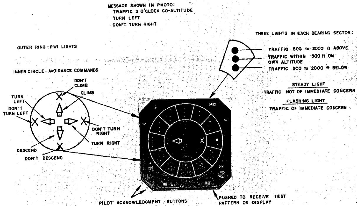
Fig.2-1. IPC display utilized in flight testing.
