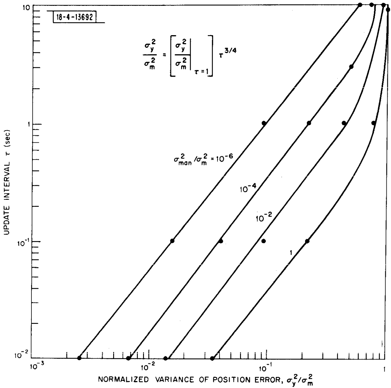
Fig. C.I. Normalized variance of position error vs update interval.
