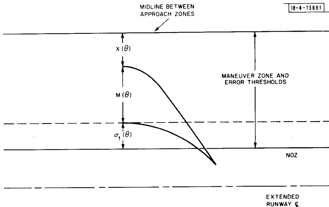
Fig. B.1. Recovery projection miss distance.
