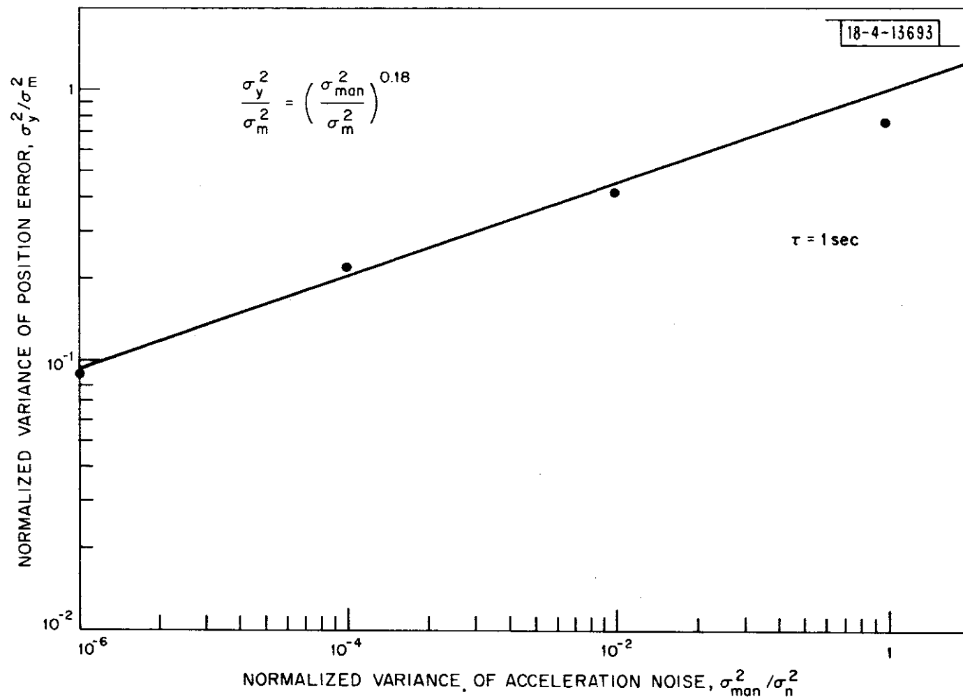
Fig. C.2. Normalized variance of position error vs normalized variance of acceleration noise.
