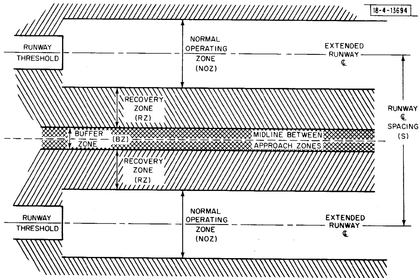
Fig. 1. Parallel runway approach zone configuration.
