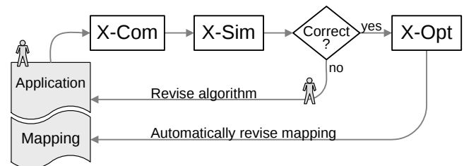
Figure 1: Design flow under Auto-Pipe
