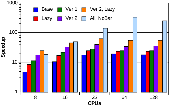
Figure 2: CEARC Performance on Loopy Belief Propagation
