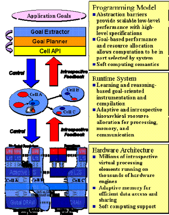
Figure 3: Summary of CEARC System Software
